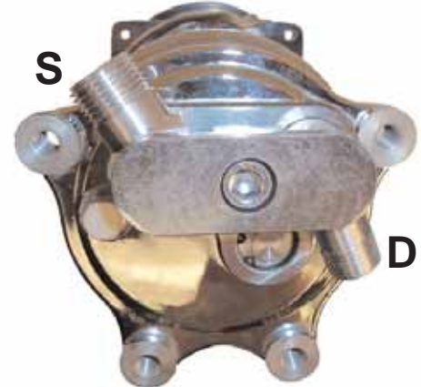
Sunair S6™ Compressor with HP-6006 Installed
